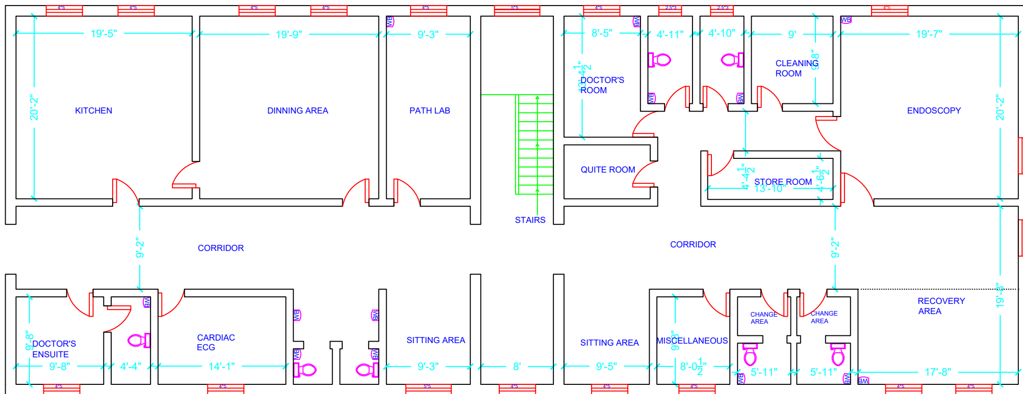
BLOCK B FIRST FLOOR (Endoscopy & Kitchen area)
