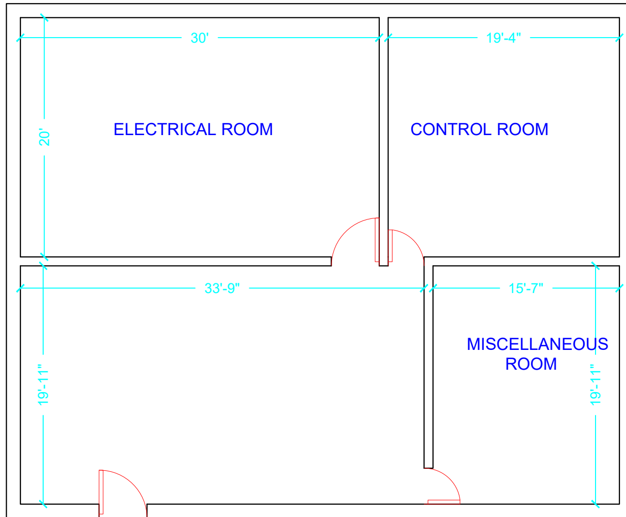
BLOCK B LOWER GROUND FLOOR (Electricity control room)
