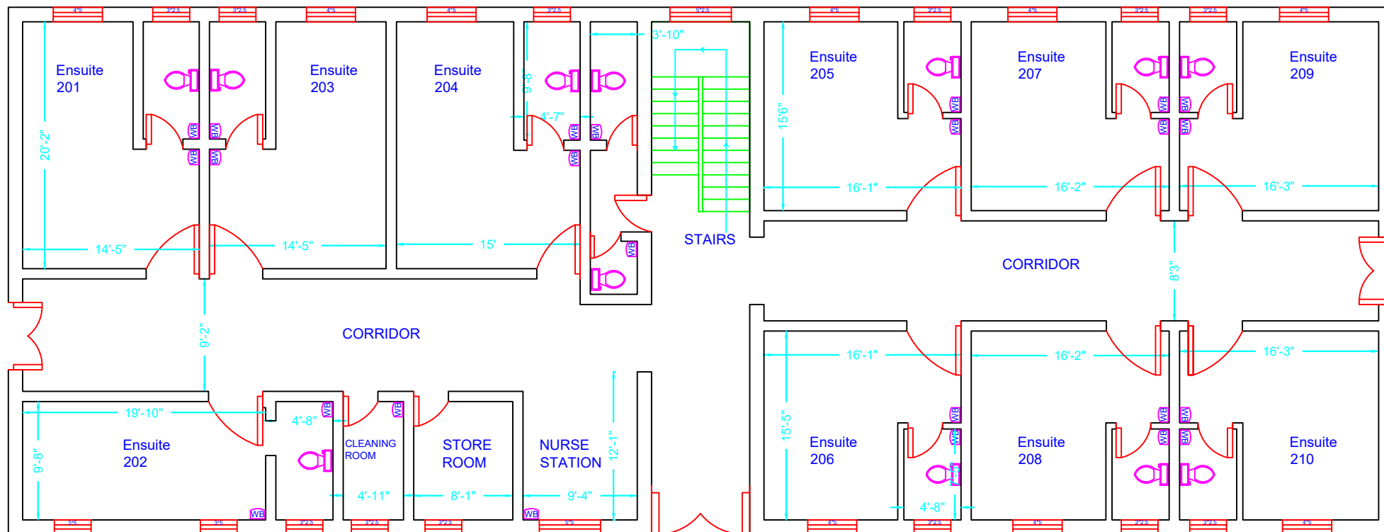
BLOCK A GROUND FLOOR (INPATIENT)
