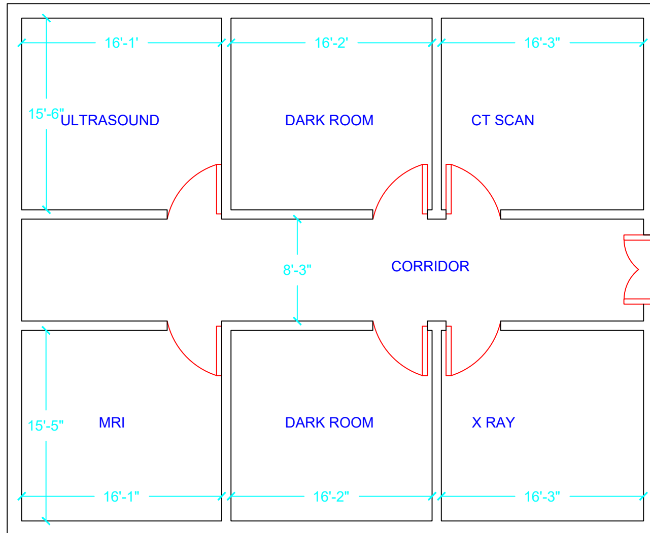
BLOCK A LOWER GROUND FLOOR (RADIOLOGY)
